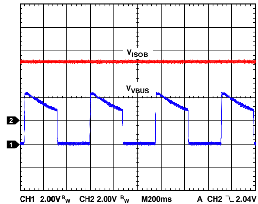
Figure 29. Battery Detection Waveform
