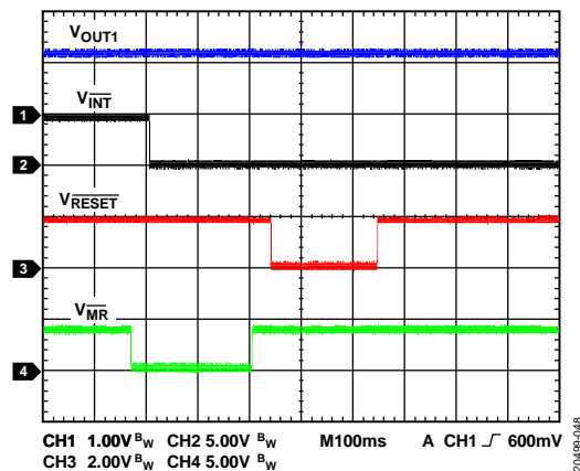
Figure 47. MR Press to Trigger Interrupt and RESET, EN_WD_INT = 1 Bit, RESET_TIME = 200ms
