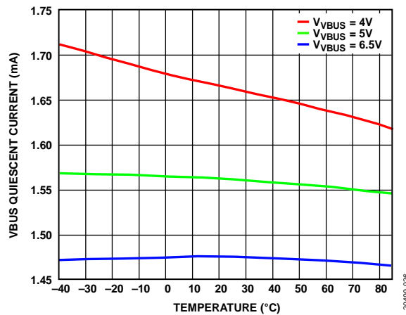
Figure 25. VBUS Quiescent Current vs. Temperature
