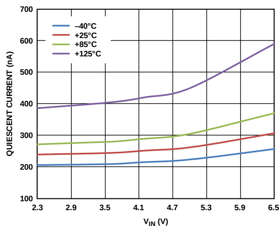
Figure 15. Hysteresis Quiescent Current vs. V_{IN} , SYNC/MODE = Low
