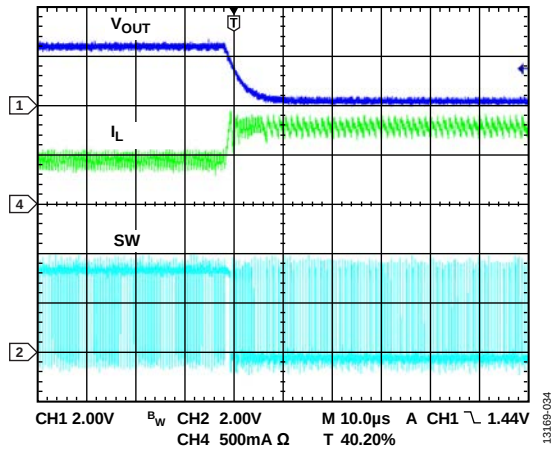
Figure 34. Output Short
