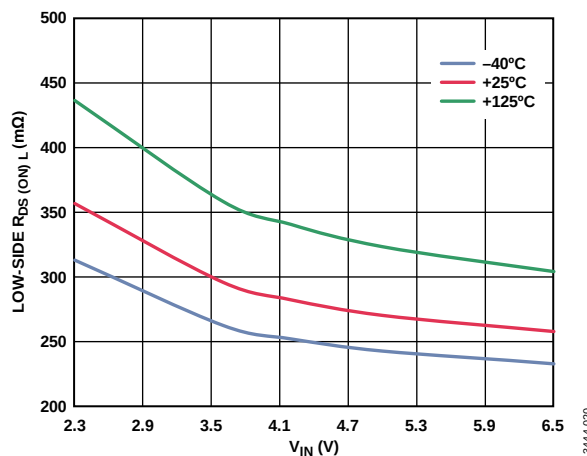
Figure 20. Low-Side R_{DS(ON)L} vs. V_{IN}
