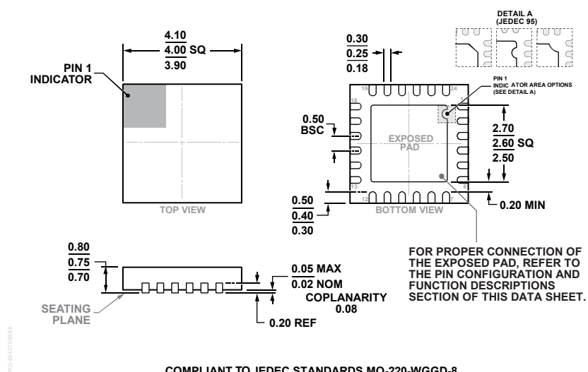
Figure 54. 24-Lead Lead Frame Chip Scale Package [LFCSP] 4 mm × 4 mm Body and 0.75 mm Package Height (CP-24-15)
