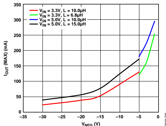
Figure 6. Maximum Output Current ( I_{OUT} ) vs. V_{NEG} for Inverting Regulator, f_{SW} = 1.2\text{ MHz} , T_A = 25^\circ\text{C} , Based on Target of 70% I_{LIM(INVERTER)}
