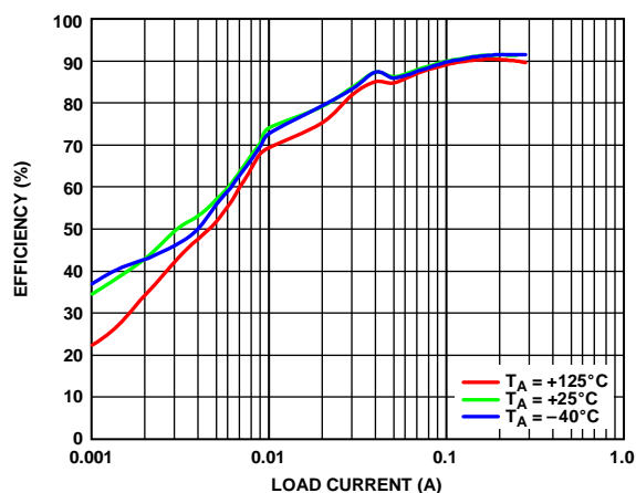
Figure 15. Efficiency vs. Load Current for Boost Regulator over Temperature, V_{IN} = 5\text{ V} , V_{POS} = 15\text{ V} , f_{SW} = 1.2\text{ MHz}
