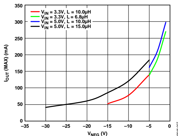
Figure 7. Maximum Output Current ( I_{OUT} ) vs. V_{NEG} for Inverting Regulator, f_{SW} = 2.4\text{ MHz} , T_A = 25^\circ\text{C} , Based on Target of 70% I_{LIM(INVERTER)}
