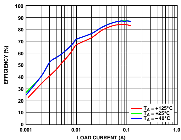
Figure 18. Efficiency vs. Load Current for Inverting Regulator over Temperature, V_{IN} = 5\text{ V} , V_{NEG} = -15\text{ V} , f_{SW} = 1.2\text{ MHz}
