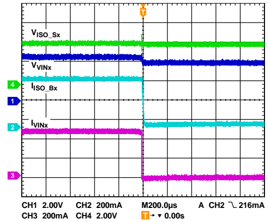
Figure 23. USB VBUS Disconnection
