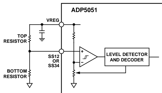
Figure 44. Level Detector Circuit for Soft Start
