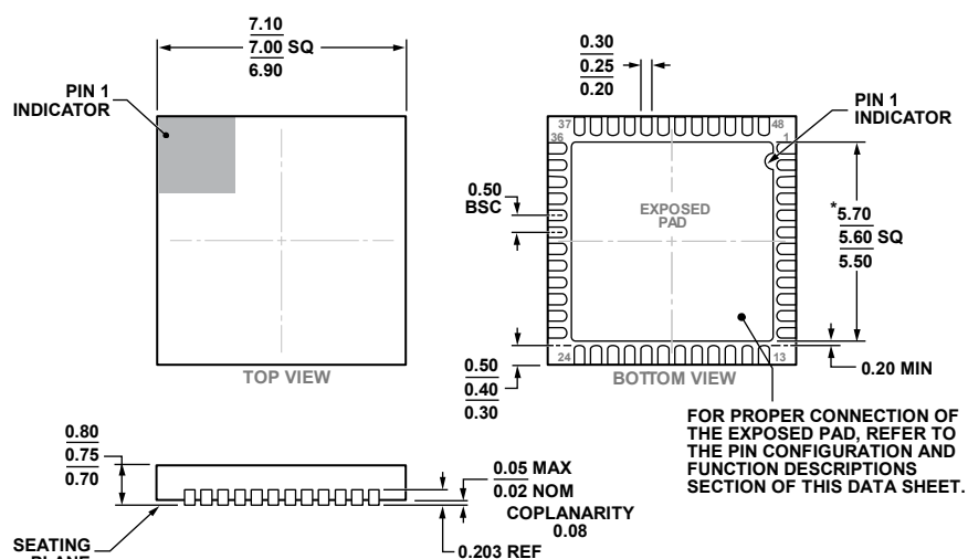
Figure 67. 48-Lead Lead Frame Chip Scale Package [LFCSP_WQ] 7 mm x 7 mm Body, Very Very Thin Quad (CP-48-13) Dimensions shown in millimeters
