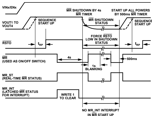
Figure 54. \overline{\text{MR}} Timing Diagram in Power-On/Off Switch Mode
