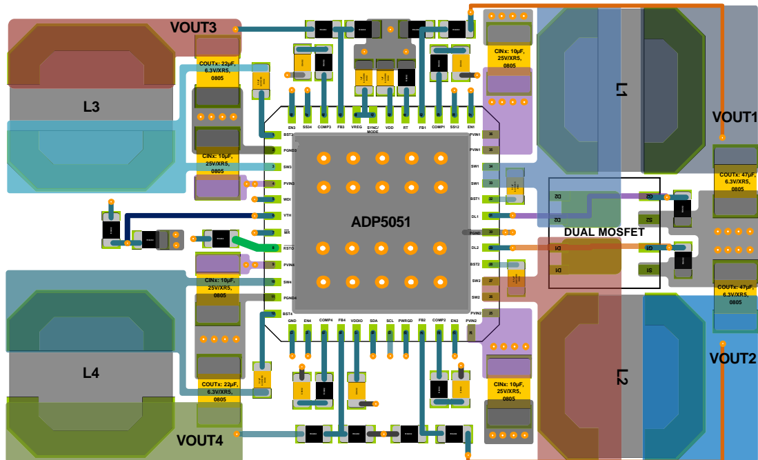
Figure 63. Typical PCB Layout
