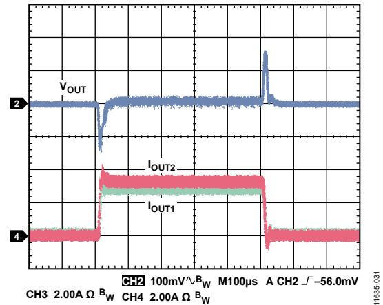
Figure 28. Load Transient, Channel 1/Channel 2 Parallel Output, 0 A to 6 A, V_{IN} = 12\text{ V} , V_{OUT} = 3.3\text{ V} , f_{SW} = 600\text{ kHz} , L = 4.7\text{ μH} , C_{OUT} = 47\text{ μF} \times 4
