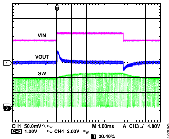
Figure 24. BUCK2 Response to Line Transient, V_{IN} = 4.5\text{ V} to 5.0 V, V_{OUT2} = 1.8\text{ V} , PWM Mode
