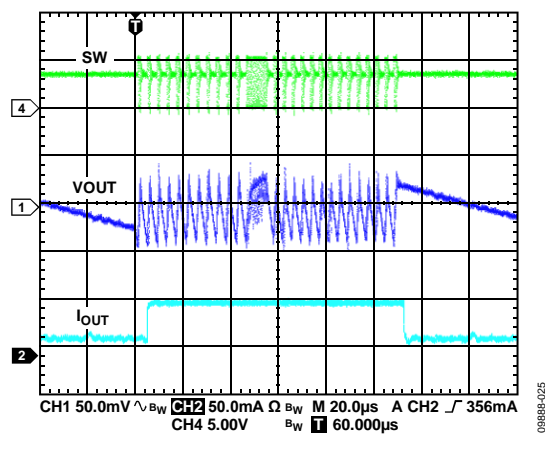
Figure 25. BUCK1 Response to Load Transient, I_{OUT1} from 1 mA to 50 mA, V_{OUT1} = 3.3\text{ V} , Automatic Mode
