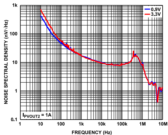
Figure 11. LDO Noise Spectral Density vs. Frequency at Various LDO Output Voltages
