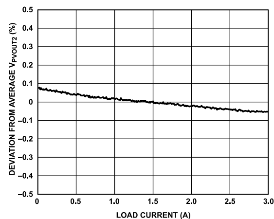
Figure 19. LDO Load Regulation, V_{PVOUT2} = 3.3\text{ V} , V_{HR} = 0.3\text{ V}
