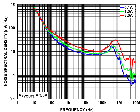
Figure 14. LDO Noise Spectral Density vs. Frequency, V_{PVOUT2} = 3.3\text{ V} at Various LDO Load Currents
