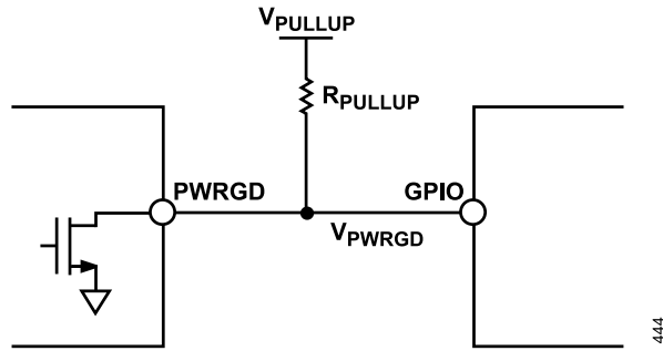
Figure 43. Power-Good Setup
