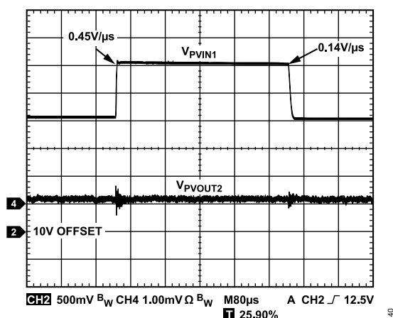
Figure 34. Adaptive Mode Line Transient, V_{PVIN1} = 11\text{ V to }13\text{ V} , V_{PVOUT2} = 3.3\text{ V} , I_{LOAD2} = 1\text{ A} , f_{SW} = 1.5\text{ MHz} , L = 2.2\text{ μH} , R_C = 3.48\text{ kΩ} , C_C = 22\text{ nF} , C_{CP} = 22\text{ pF} , C_{PVOUT1} = 64\text{ μF}
