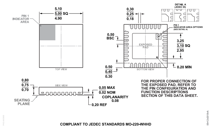
Figure 54. 32-Lead Lead Frame Chip Scale Package [LFCSP] 5 mm x 5 mm Body and 0.75 mm Package Height (CP-32-7) Dimensions shown in millimeters
