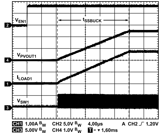
Figure 39. Buck Startup
