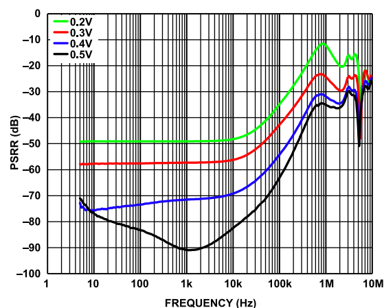
Figure 13. LDO PSRR vs. Frequency, V_{PVOUT2} = 3.3\text{ V} , I_{LOAD2} = 1\text{ A} at Various LDO Headroom Voltages
