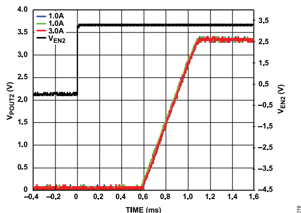
Figure 41. LDO Startup
