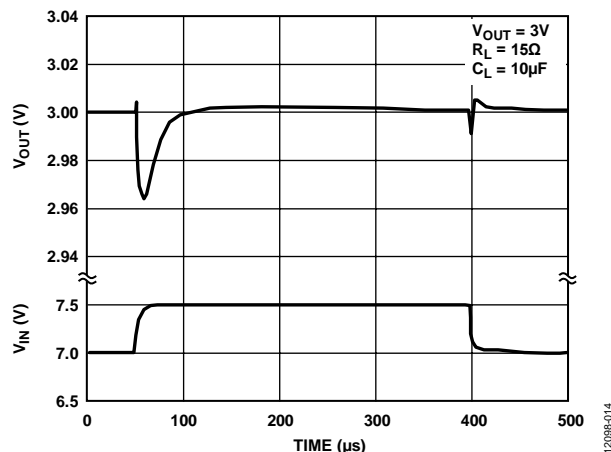
Figure 14. Line Transient Response, C_L = 10 \mu\text{F}
