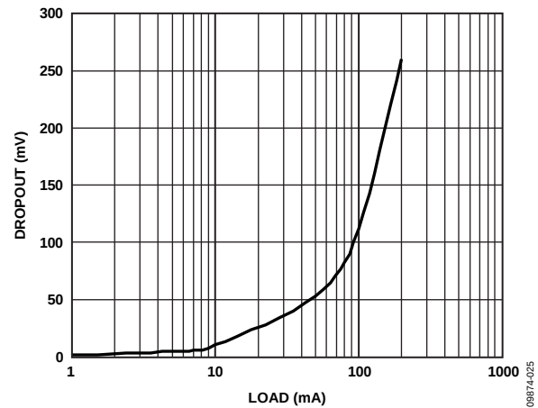
Figure 25. Dropout Voltage vs. Load Current and Output Voltage, V_{OUT2} = 1.8 \text{ V} , V_{RIPPLE} = 50 \text{ mV} , C_{OUT} = 1 \mu\text{F}
