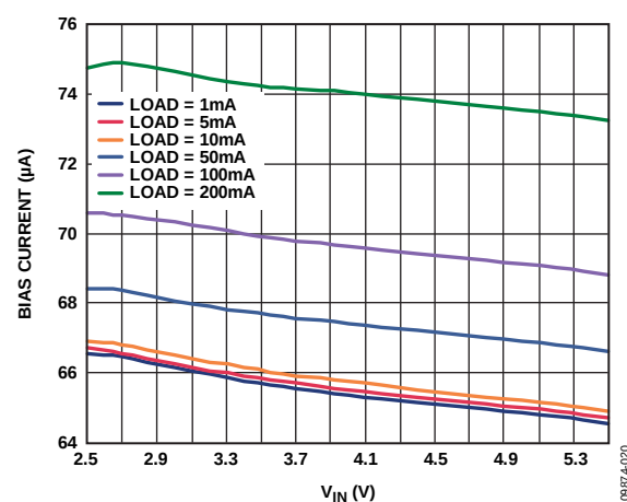
Figure 20. Bias Current vs. Input Voltage, Single Output Load, V_{\text{RIPPLE}} = 50 \text{ mV} , C_{\text{OUT}} = 1 \mu\text{F}
