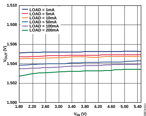
Figure 11. Output Voltage vs. Input Voltage, V_{\text{RIPPLE}} = 50 \text{ mV} , C_{\text{OUT}} = 1 \mu\text{F}
