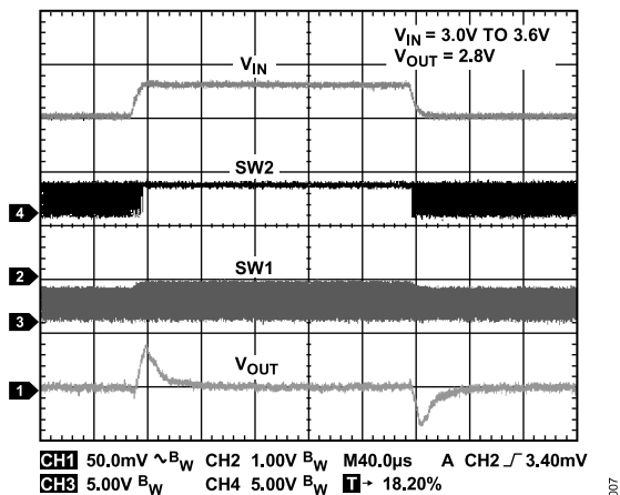
Figure 17. Line Transient, PWM Mode ( V_{IN} = 3.0 V to 3.6 V, V_{OUT} = 2.8 V)
