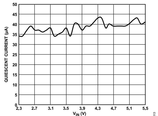
Figure 14. Quiescent Current vs. Input Voltage ( V_{OUT} = 3.3 V)
