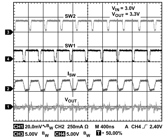
Figure 24. Typical PWM Switching Waveform, Buck-Boost Operation ( V_{OUT} = 3.3\text{ V} )
