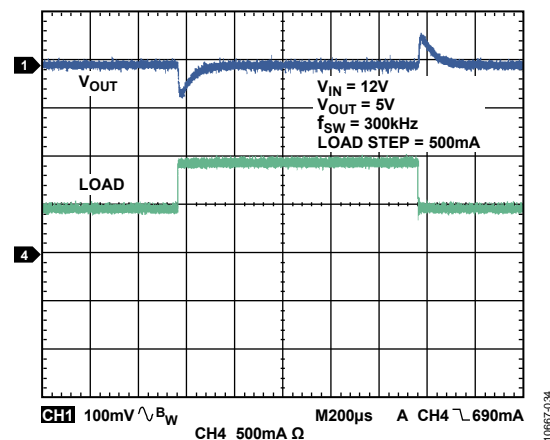
Figure 39. Load Transient Response,
