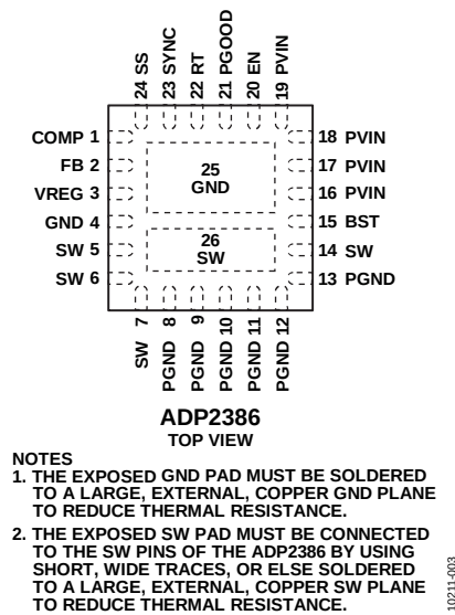
Figure 3. Pin Configuration
