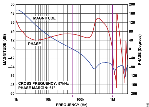
Figure 29. Bode Plot at V_{IN} = 5\text{ V} , V_{OUT} = 1.0\text{ V} , I_O = 4\text{ A} , f_S = 1.2\text{ MHz} , L = 0.68\text{ }\mu\text{H} , C_{OUT} = 2 \times 100\text{ }\mu\text{F}
