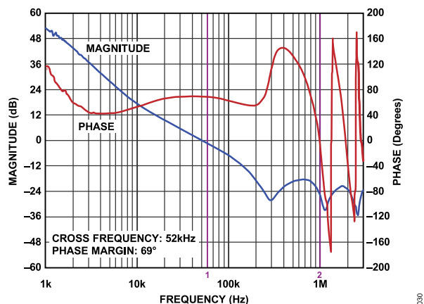
Figure 30. Bode Plot at V_{IN} = 5\text{ V} , V_{OUT} = 1.5\text{ V} , I_O = 4\text{ A} , f_S = 1.2\text{ MHz} , L = 1\text{ }\mu\text{H} , C_{OUT} = 47\text{ }\mu\text{F} + 100\text{ }\mu\text{F}
