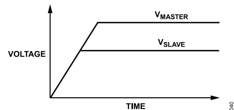
Figure 40. Coincident Tracking
