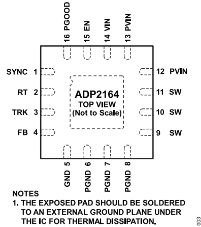
Figure 3. Pin Configuration
