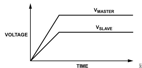
Figure 41. Ratiometric Tracking
