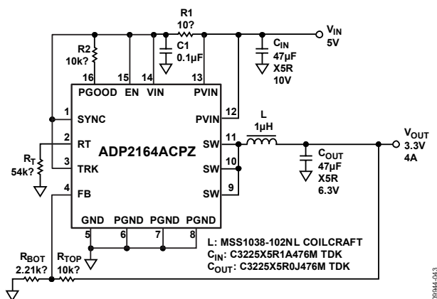
Figure 45. 3.3 V, 4 A, 1 MHz Step-Down Regulator
