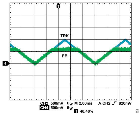
Figure 28. Tracking Function
