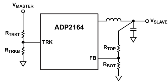
Figure 39. Voltage Tracking
