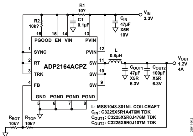
Figure 42. 1.2 V, 4 A, 1.2 MHz Step-Down Regulator
