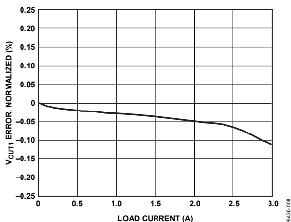
Figure 8. Load Regulation, Channel 1: V_{IN} = 5 V, f_{SW} = 600 kHz, and T_A = 25^\circ\text{C}
