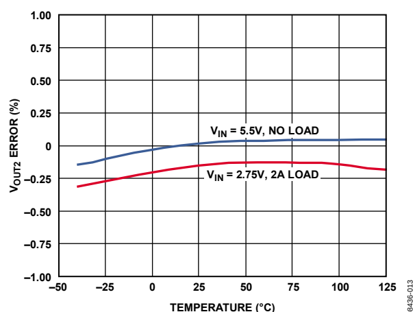
Figure 13. Output Voltage Error vs. Temperature, Channel 2: V_{OUT} = 1.5 V and f_{SW} = 600 kHz
