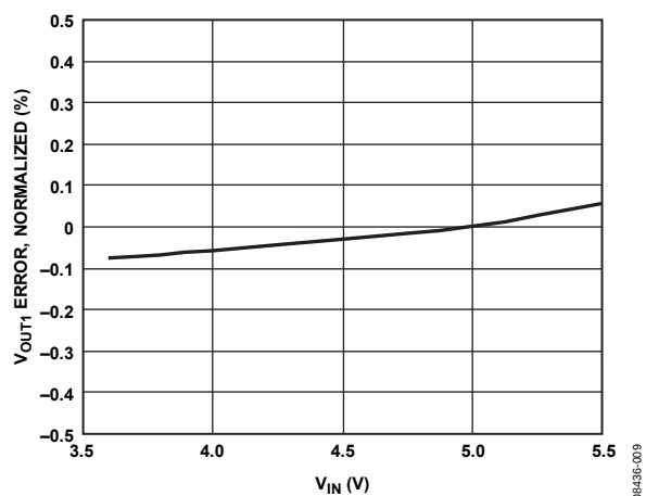
Figure 9. Line Regulation, Channel 1: Load Current = 3 A and f_{SW} = 600 kHz
