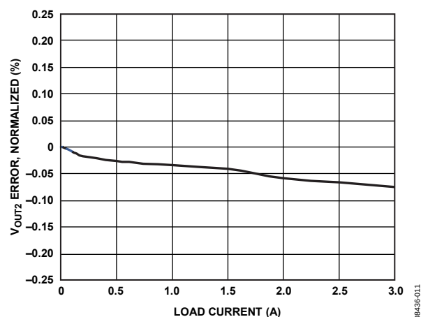
Figure 11. Load Regulation, Channel 2: V_{IN} = 5 V, f_{SW} = 600 kHz, and T_A = 25^\circ\text{C}
