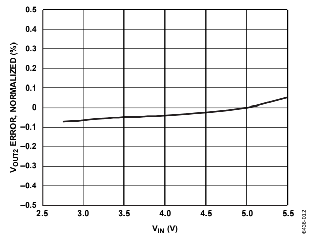
Figure 12. Line Regulation, Channel 2: Load Current = 3 A and f_{SW} = 600 kHz
