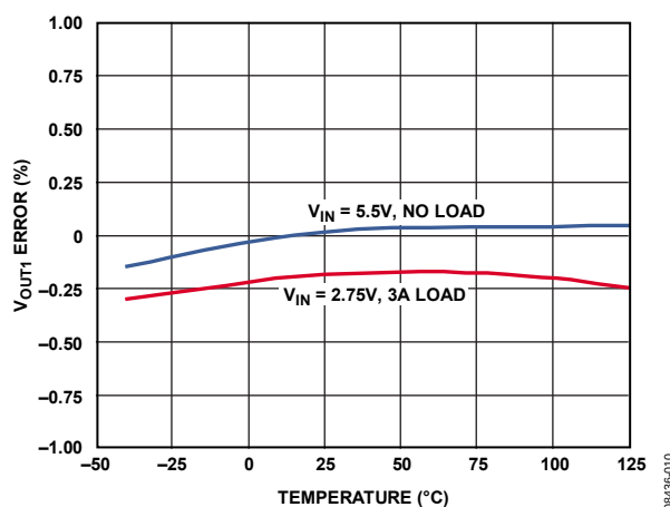
Figure 10. Output Voltage Error vs. Temperature, Channel 1: V_{OUT} = 0.6 V and f_{SW} = 600 kHz
