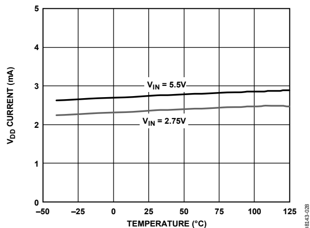
Figure 28. VDD Input Current vs. Temperature (Not Switching)
