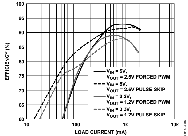
Figure 6. Efficiency vs. Load at f_{SW} = 1.2MHz ; Inductor TOKO FDV0620-1R0M, 1.0\mu H , 14m\Omega
