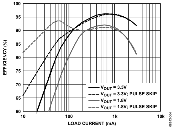
Figure 4. Channel 1 Efficiency vs. Load, V_{IN} = 5V and f_{SW} = 300kHz ; V_{OUT} = 3.3V , Inductor Cooper Bussmann DR1050-8R2-R, 8.2\mu H , 15m\Omega ; V_{OUT} = 1.8V , Inductor TOKO FDV0620-4R7M, 4.7\mu H , 53m\Omega
