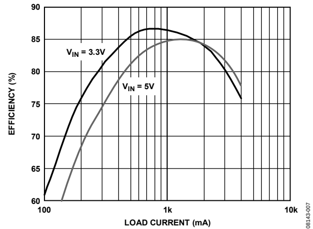
Figure 7. Efficiency Combined Dual-Phase Output, V_{OUT} = 0.8V and f_{SW} = 1.2MHz ; Inductor TOKO FDV0620-1R0M, 1.0\mu H , 14m\Omega
