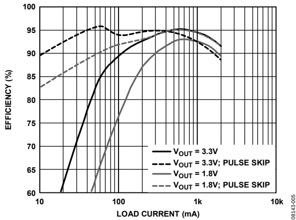
Figure 5. Channel 2 Efficiency vs. Load, V_{IN} = 5V and f_{SW} = 600kHz ; V_{OUT} = 3.3V , Inductor TOKO FDV0620-4R7M, 4.7\mu H , 53m\Omega ; V_{OUT} = 1.8V , Inductor TOKO FDV0620-2R2M, 2.2\mu H , 30m\Omega
