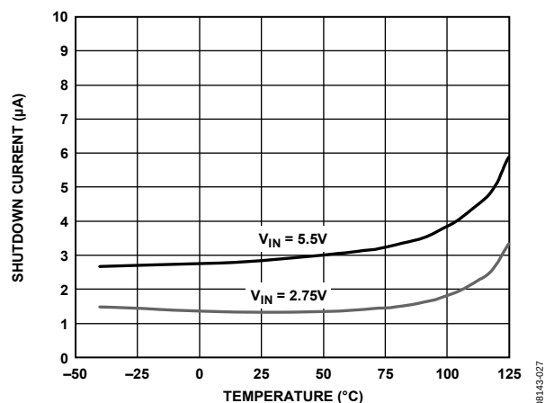
Figure 27. Shutdown Current vs. Temperature
