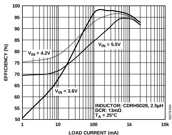
Figure 12. Efficiency—ADP2107 (3.3 V)
