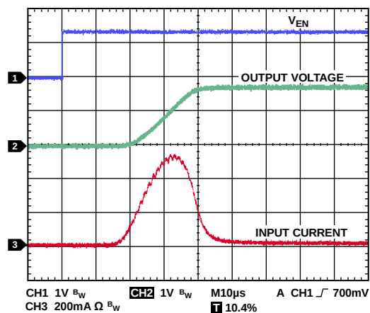
Figure 25. Typical Turn-On Time and Inrush Current, V_{IN} = 1.8V , 10 mA Load, C_{OUT} = 4.7\mu F
