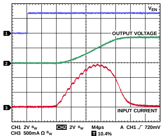
Figure 27. Typical Turn-On Time and Inrush Current, V_{IN} = 3.6V , 10 mA Load, C_{OUT} = 4.7\mu F
