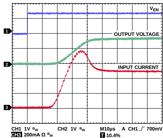
Figure 26. Typical Turn-On Time and Inrush Current, V_{IN} = 1.8V , 500 mA Load, C_{OUT} = 4.7\mu F
