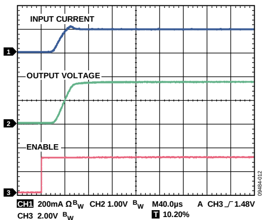
Figure 12. Typical Rise Time and Inrush Current, V_{IN} = 1.8V , I_{LOAD} = 200mA , Select Code 00
