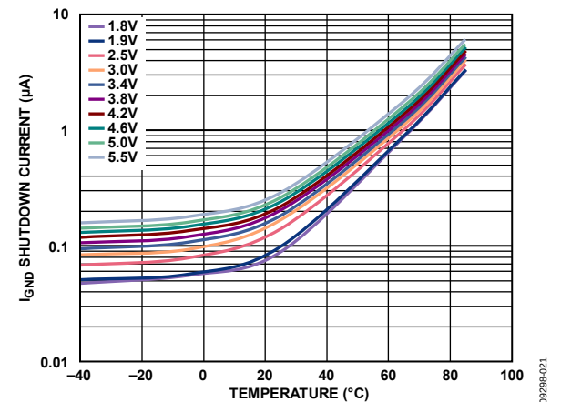
Figure 15. I_{GND} Shutdown Current vs. Temperature, V_{OUT} = 0\text{ V} , Different Input Voltages ( V_{IN} )
