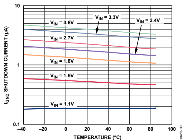
Figure 13. Reverse Shutdown Current vs. Temperature, V_{OUT} = 0 V
