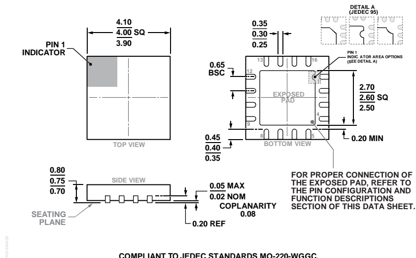
Figure 36. 16-Lead Lead Frame Chip Scale Package [LFCSP] 4 mm × 4 mm Body and 0.75 mm Package Height (CP-16-17) Dimensions shown in millimeters
