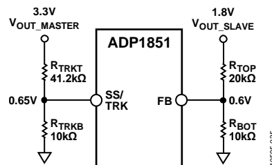
Figure 33. Example of a Ratiometric Tracking Circuit
