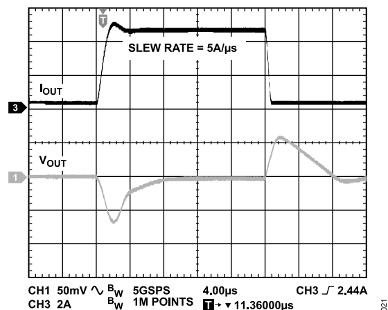
Figure 21. Load Transient Response, C_{OUT} = 47\text{ }\mu\text{F} , V_{IN} = 1.8\text{ V} , V_{OUT} = 1.3\text{ V}
