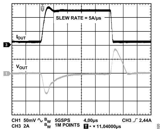
Figure 20. Load Transient Response, C_{OUT} = 22\text{ }\mu\text{F} , V_{IN} = 1.8\text{ V} , V_{OUT} = 1.3\text{ V}
