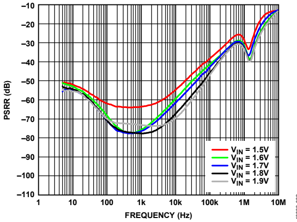
Figure 32. Power Supply Rejection Ratio (PSRR) vs. Frequency at Various Input Voltages ( V_{in} ), V_{out} = 1.3\text{ V} , Load = 5 A
