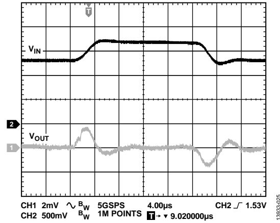
Figure 25. Line Transient Response, Load Current = 5 A, V_{IN} = 1.3 V to 1.7 V Step, V_{OUT} = 0.9 V
