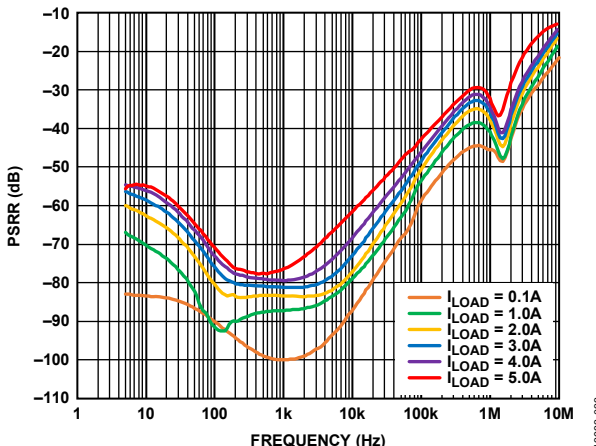
Figure 33. Power Supply Rejection Ratio (PSRR) vs. Frequency at Various Loads ( I_{load} ), V_{out} = 1.3\text{ V} , V_{in} = 1.7\text{ V}
