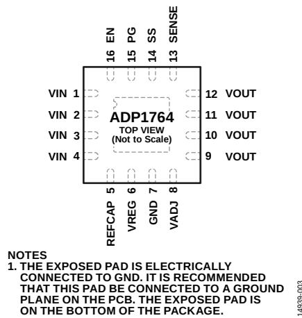
Figure 3. Pin Configuration
