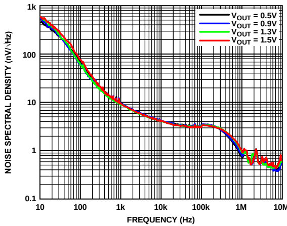
Figure 29. Noise Spectral Density vs. Frequency at Various Output Voltages ( V_{OUT} ), 10 Hz to 10 MHz
