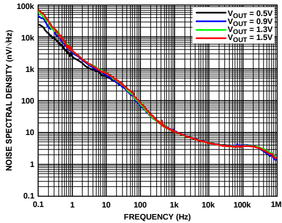
Figure 28. Noise Spectral Density vs. Frequency at Various Output Voltages ( V_{OUT} ), 0.1 Hz to 1 MHz
