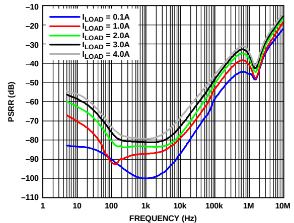
Figure 33. Power Supply Rejection Ratio (PSRR) vs. Frequency at Various Loads ( I_{LOAD} ), V_{OUT} = 1.3 V, V_{IN} = 1.7 V
