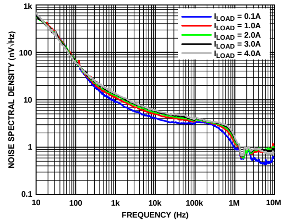
Figure 31. Noise Spectral Density vs. Frequency at Various Load Current ( I_{LOAD} ), 10 Hz to 10 MHz
