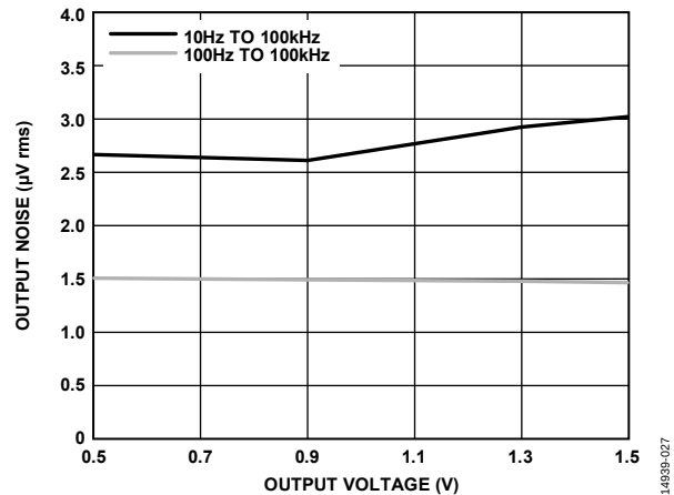
Figure 27. Output Noise vs. Output Voltage ( V_{OUT} )
