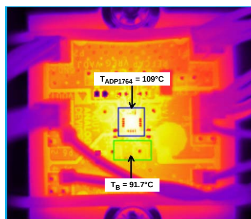
Figure 56. Thermal Image of the ADP1764 Evaluation Board at I_{\text{LOAD}} = 4 \text{ A} , V_{IN} = 1.5 \text{ V} , V_{OUT} = 1.3 \text{ V} , T_B = 91.7^{\circ}\text{C}
