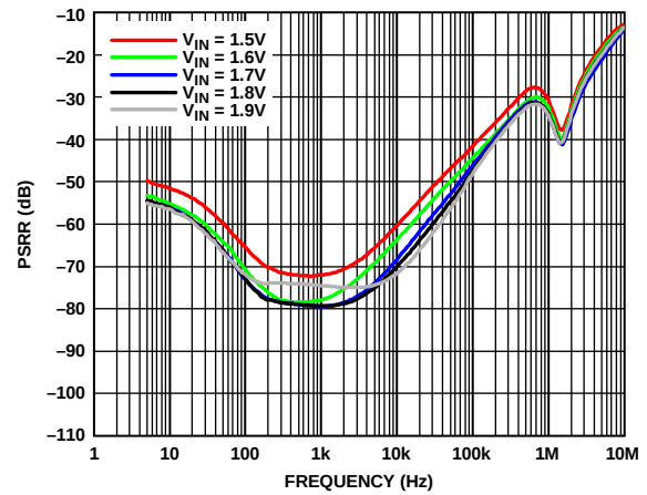
Figure 32. Power Supply Rejection Ratio (PSRR) vs. Frequency at Various Input Voltages ( V_{IN} ), V_{OUT} = 1.3 V, Load = 4 A
