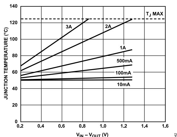
Figure 44. 1000 \text{mm}^2 of PCB Copper, T_B = 50^{\circ}\text{C} , LFCSP
