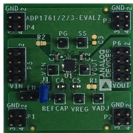
Figure 46. Evaluation Board
