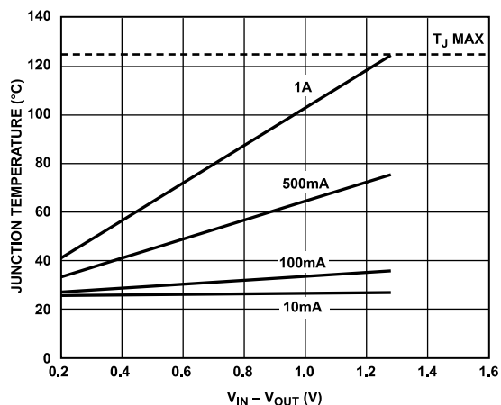
Figure 35. 500 \text{mm}^2 of PCB Copper, T_A = 25^{\circ}\text{C}
