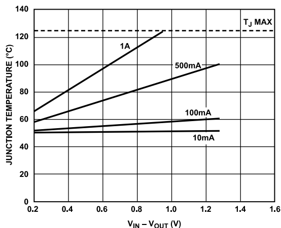
Figure 38. 500 \text{mm}^2 of PCB Copper, T_A = 50^{\circ}\text{C}
