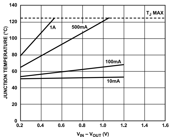
Figure 39. 25 \text{mm}^2 of PCB Copper, T_A = 50^{\circ}\text{C}
