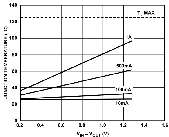
Figure 34. 6400 \text{mm}^2 of PCB Copper, T_A = 25^{\circ}\text{C}
