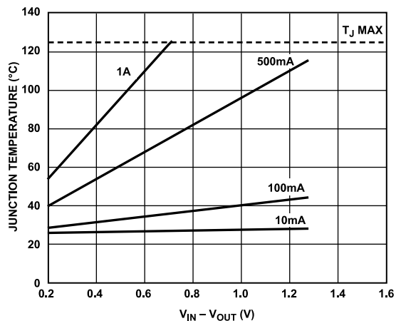
Figure 36. 25 \text{mm}^2 of PCB Copper, T_A = 25^{\circ}\text{C}
