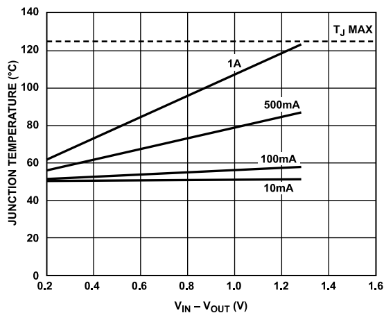
Figure 37. 6400 \text{mm}^2 of PCB Copper, T_A = 50^{\circ}\text{C}
