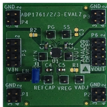
Figure 44. Evaluation Board
