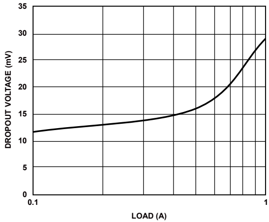
Figure 11. Dropout Voltage vs. Load Current, V_{OUT} = 1.3 V
