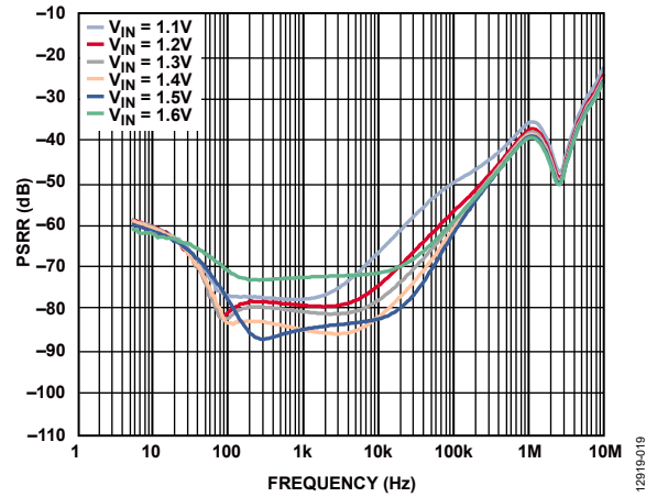
Figure 19. Power Supply Rejection Ratio (PSRR) vs. Frequency for Various V_{IN} , V_{OUT} = 0.9 V, Load Current = 1 A
