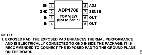
Figure 8. 8-Lead SOIC, ADP1708
