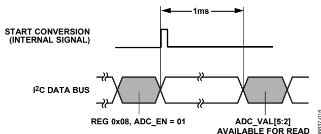
Figure 38. ADC Timing for All Modes Except V_F Measurement in Flash Mode
