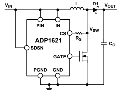
Figure 28. CS Pin Connection for V_{SW} < 30 V, Lossless Mode (No Current-Sense Resistor Needed)
