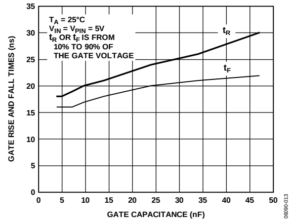
Figure 14. GATE Rise and Fall Times vs. C_{GATE}
