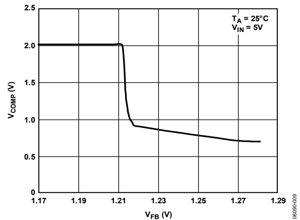
Figure 10. V_{\text{COMP}} vs. V_{\text{FB}}
