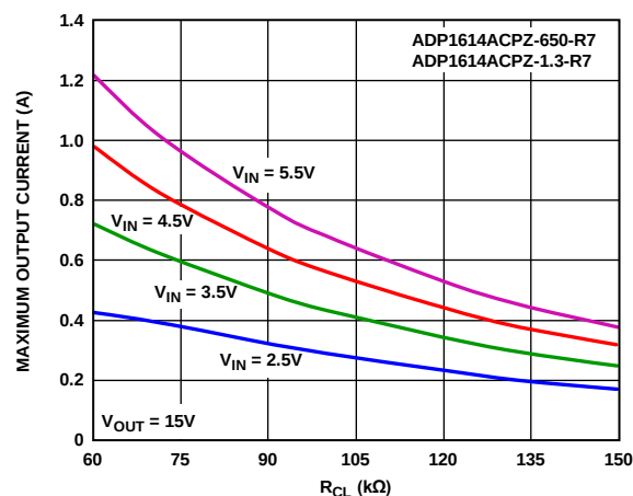
Figure 9. Typical Maximum Continuous Output Current vs. R_{CL} , V_{OUT} = 15V
