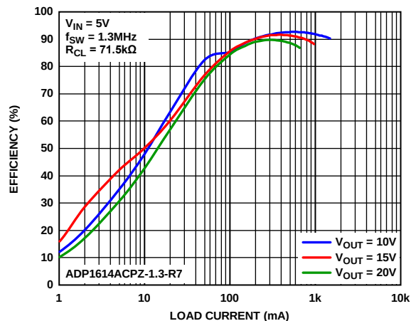
Figure 7. Efficiency vs. Load Current, V_{IN} = 5V , f_{SW} = 1.3MHz
