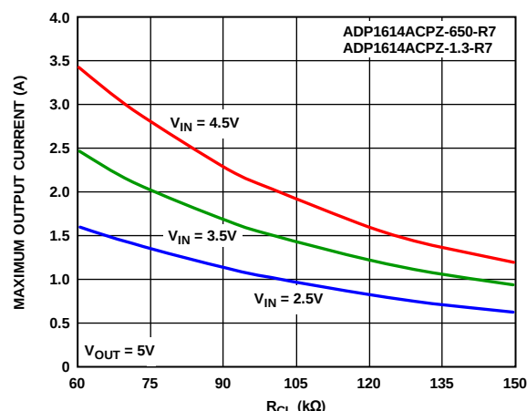
Figure 8. Typical Maximum Continuous Output Current vs. R_{CL} , V_{OUT} = 5V
