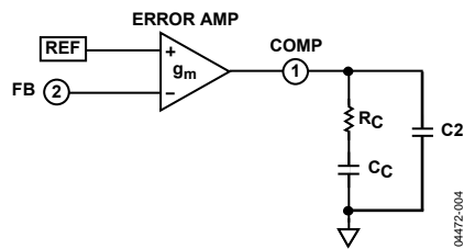
Figure 26. Compensation Components
