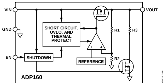
Figure 30. Internal Block Diagram, Fixed Output with Output Discharge Function
