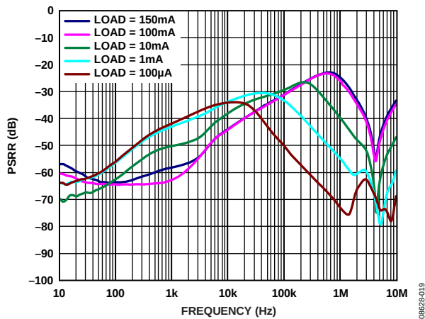
Figure 19. Power Supply Rejection Ratio vs. Frequency, V_{OUT} = 3.3\text{ V} , V_{IN} = 4.3\text{ V}
