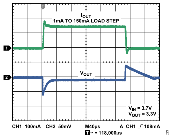
Figure 23. Load Transient Response, C_{OUT} = 4.7 \mu F
