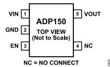
Figure 3. 5-Lead TSOT Pin Configuration
