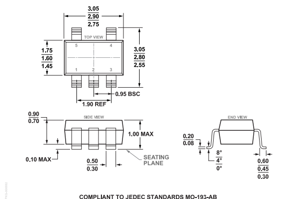
Figure 49. 5-Lead Thin Small Outline Transistor Package [TSOT] (UJ-5) Dimensions shown in millimeters
