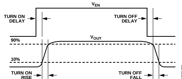
Figure 2. Timing Diagram
