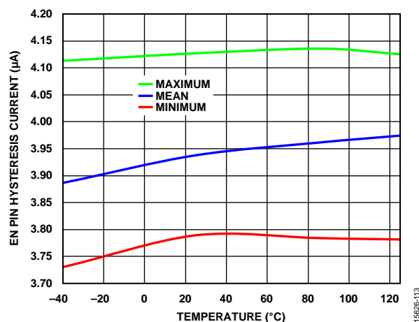
Figure 15. EN Pin Hysteresis Current vs. Temperature, EN &lt; 1.2 V
