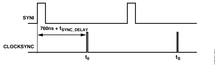
Figure 65. Synchronization Timing
