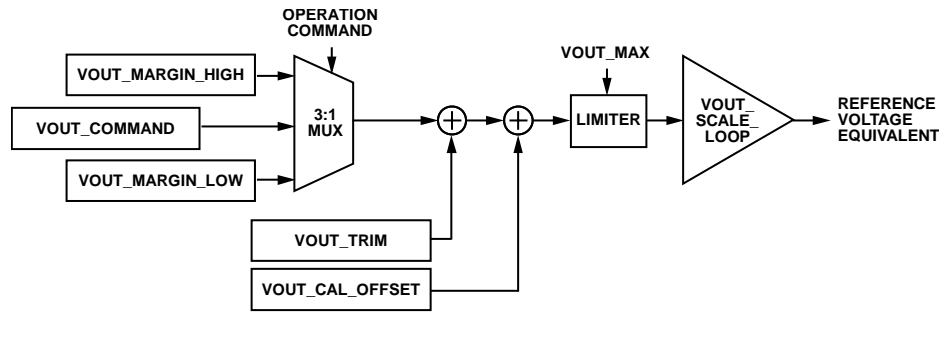
Figure 53. Conceptual View of the Output Voltage Related Commands
