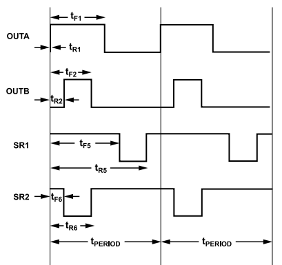
Figure 58. PWM Timing Diagram
