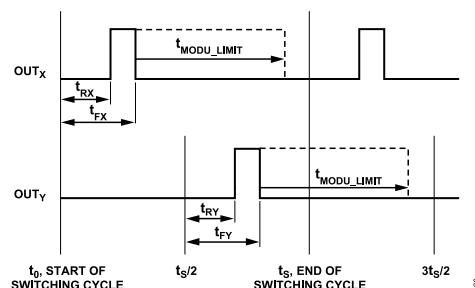
Figure 57. Setting Modulation Limits
