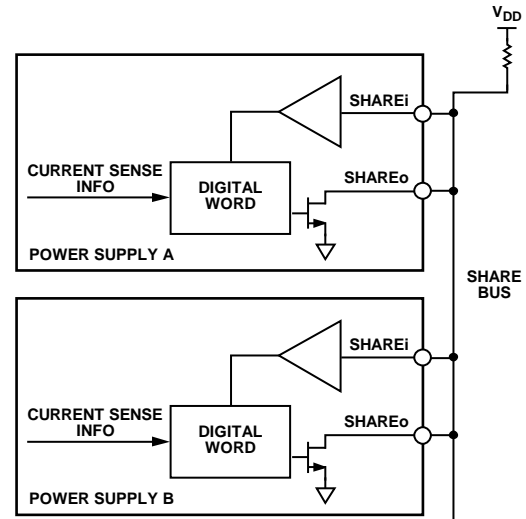
Figure 22. Digital Current Share Configuration
