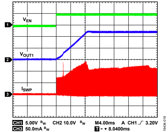
Figure 19. Inrush Current, T_A = +25^\circ\text{C} , V_{INP} = +24\text{ V} , V_{OUT1} = +24\text{ V} , I_{OUT1} = +20\text{ mA} , V_{OUT2} = +5.15\text{ V} , I_{OUT2} = +7\text{ mA} , V_{OUT3} = -15\text{ V} , I_{OUT3} = -0.3\text{ mA}
