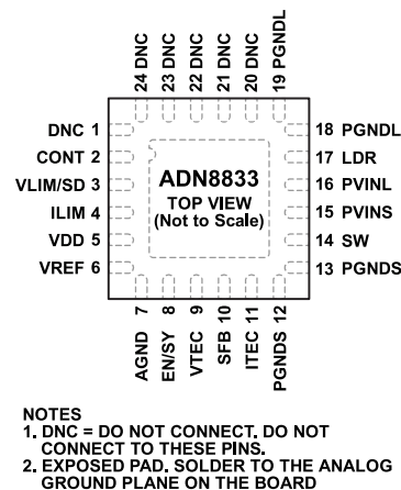
Figure 3. LFCSP Pin Configuration (Top View)
