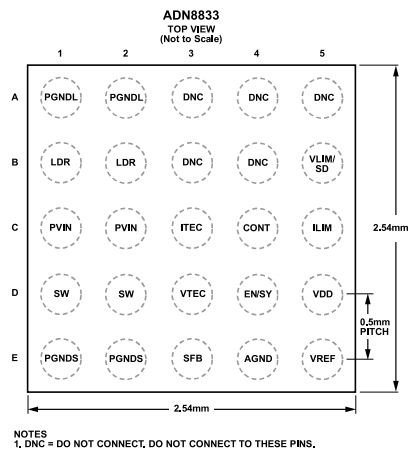
Figure 2. WLCSP Pin Configuration (Top View)
