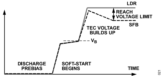
Figure 27. Soft Start Profile in Cooling Mode
