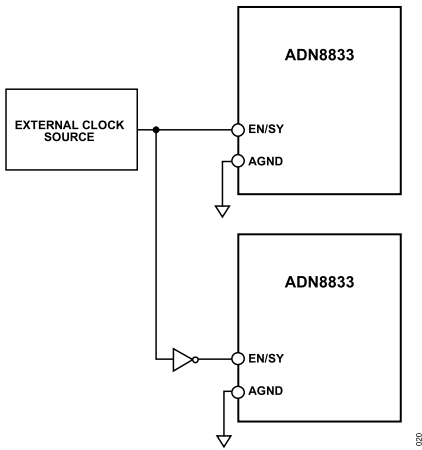
Figure 26. Multiple ADN8833 Devices Driven from a Controller Clock
