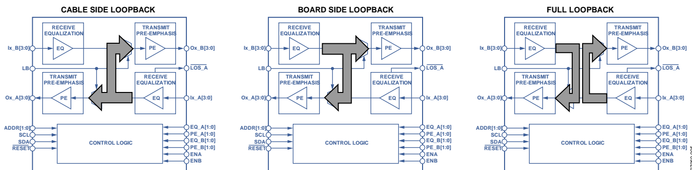
Figure 40. Loopback Modes of Operation
