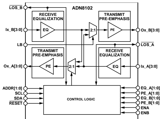
Figure 38. Simplified Functional Block Diagram
