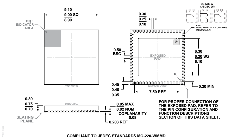
Figure 49. 64-Lead Lead Frame Chip Scale Package [LFCSP] 9 mm × 9 mm Body and 0.75 mm Package Height (CP-64-17)
