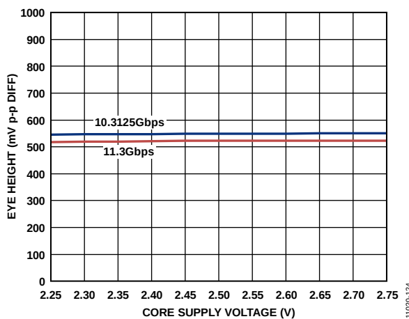
Figure 11. Eye Height vs. Core Supply Voltage ( V_{CC} )
