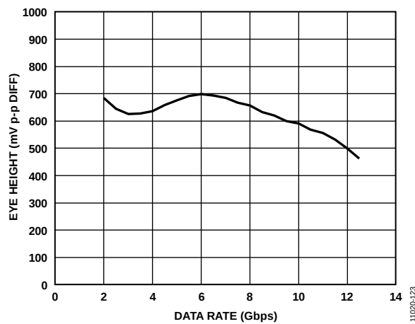
Figure 10. Eye Height vs. Data Rate
