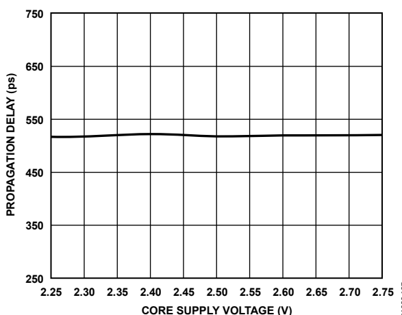
Figure 24. Propagation Delay vs. Core Supply Voltage ( V_C )
