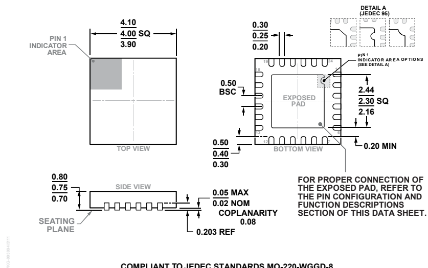
Figure 34. 24-Lead Lead Frame Chip Scale Package [LFCSP]
