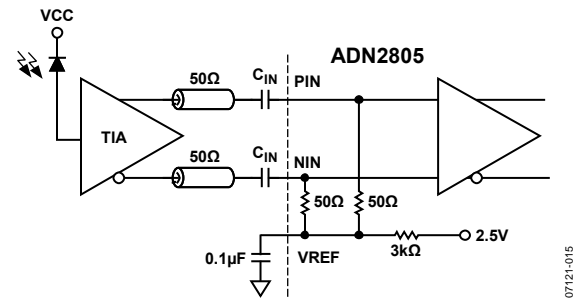
Figure 15. AC-Coupled Input Configuration
