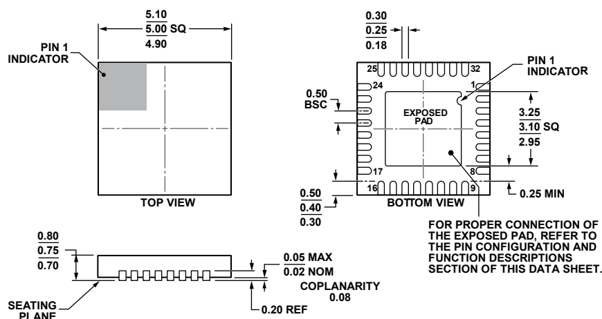
Figure 17. 32-Lead Lead Frame Chip Scale Package [LFCSP_WQ] 5 mm × 5 mm Body, Very Thin Quad (CP-32-7)
