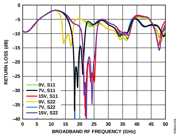
Figure 28. Return Loss vs. Broadband RF Frequency for Various VTUNE Voltages
