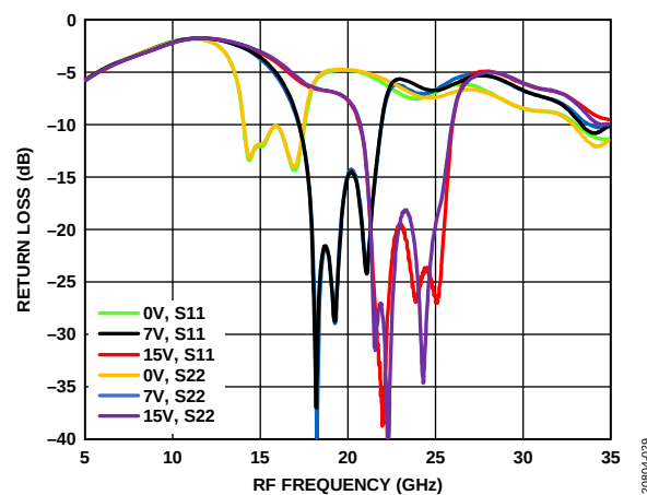
Figure 29. Return Loss vs. RF Frequency for Various VTUNE Voltages
