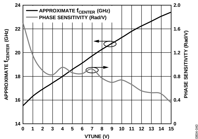
Figure 40. Approximate f_{\text{CENTER}} and Phase Sensitivity vs. VTUNE
