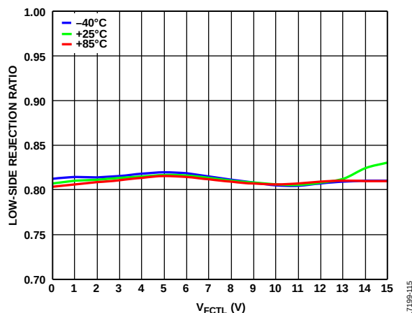
Figure 15. Low-Side Rejection Ratio vs. V_{\text{FCTL}} at Various Temperatures
