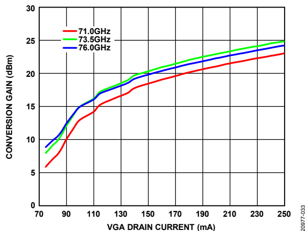
Figure 33. Conversion Gain vs. VGA Current at Various RF Frequencies, VGA\_CTL12 = -1\text{ V}
