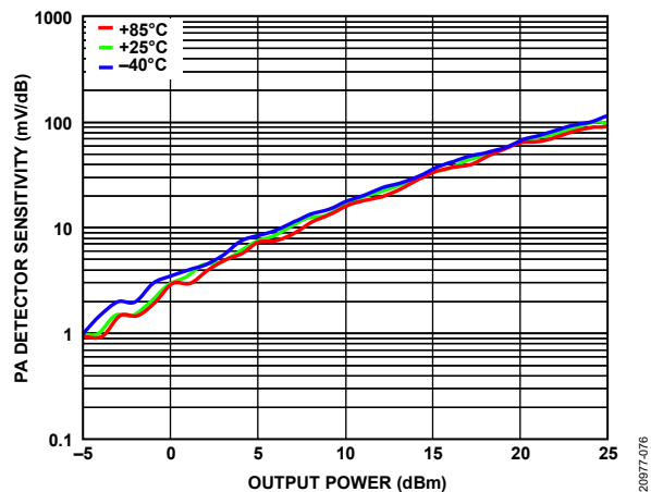
Figure 75. PA Detector Sensitivity vs. Output Power over Temperature, RF = 71 GHz
