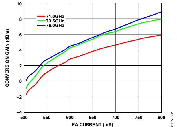
Figure 32. Conversion Gain vs. PA Current at Various RF Frequencies, VGA\_CTL12 = -1V , VGA\_VD12 = 75mA , VGA\_VD345 = 75mA , VGA\_VD6 = 75mA
