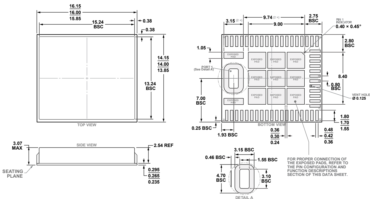
Figure 87. 50-Terminal Chip Array Small Outline No Lead Cavity [LGA_CAV] 16.00 mm x 14.00 mm Body and 3.07 mm Package Height (CE-50-2) Dimensions shown in millimeters
