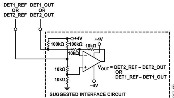
Figure 83. Typical Application Circuit for Power Detector
