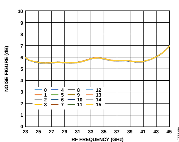
Figure 82. Noise Figure vs. RF Frequency at Different IF_AMP_FINE_GAIN_x Settings, f_{IF} = 3.5 GHz (Upper Sideband); Settings for Register 0x08, Bits[7:4] and Bits[3:0] Are the Same
