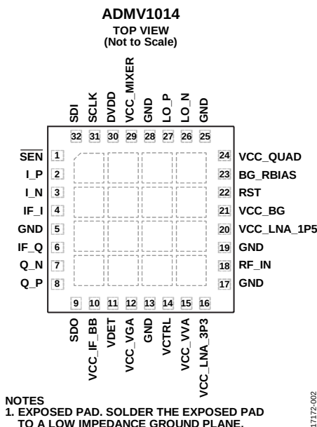
Figure 3. Pin Configuration
