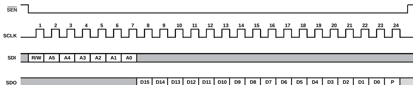
Figure 104. Read Serial Port Timing Diagram
