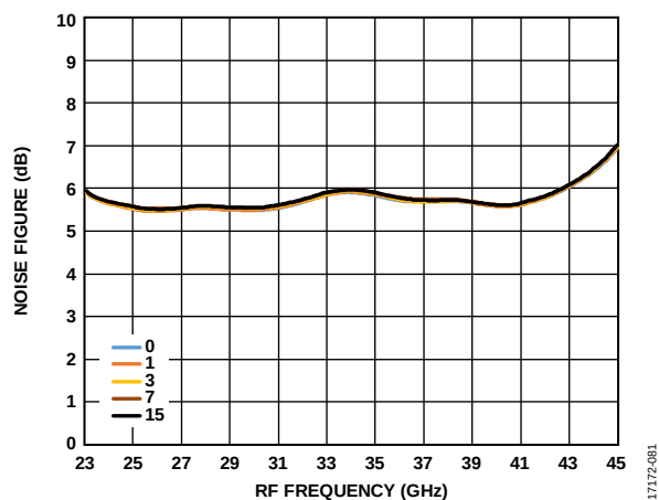
Figure 79. Noise Figure vs. RF Frequency at Different IF_AMP_COARSE_GAIN_x Settings, f_{IF} = 3.5 GHz (Upper Sideband); Settings for Register 0x08, Bits[11:8] and Register 0x09, Bits[15:12] Are the Same
