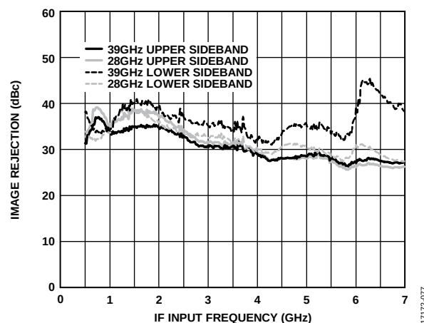
Figure 75. Image Rejection vs. IF Input Frequency at Maximum Gain, f_{RF} = 28 GHz and 39 GHz (Upper Sideband and Lower Sideband)
