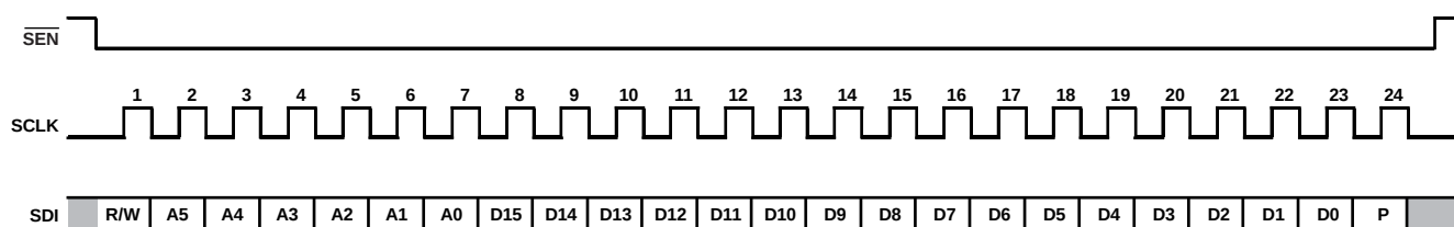
Figure 103. Write Serial Port Timing Diagram
